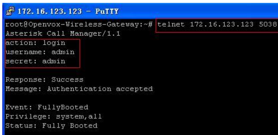
Figure 8-1-2 Putty Access
