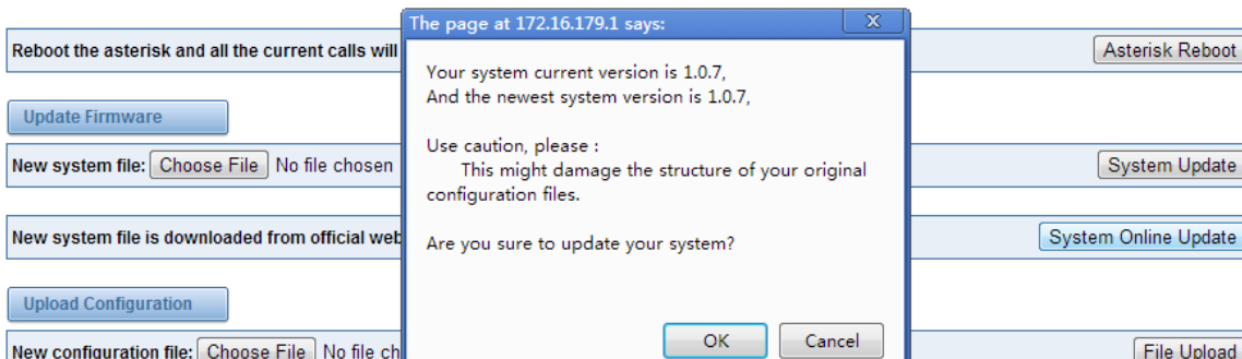
Figure 2-5-2 Prompt Information
